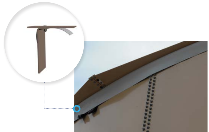
» Unique liner attachment wind girder with fin neck bolts
